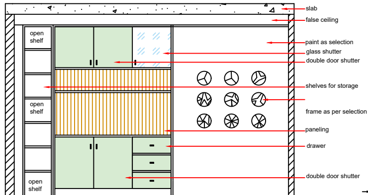
ELEVATION WITH DETAIL
