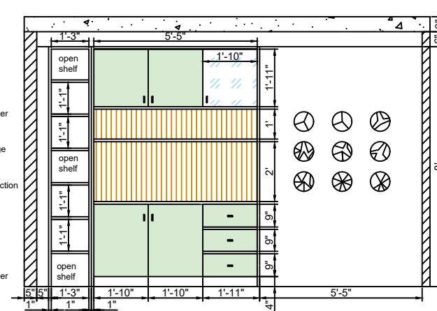
ELEVATION WITH DIMENTION
