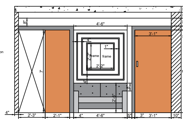
ELEVATION WITH DIMENTION
