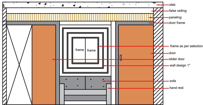
ELEVATION WITH DETAIL
