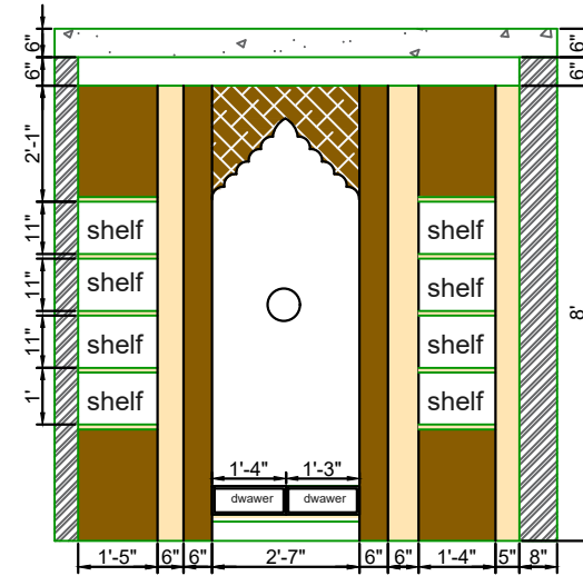
ELEVATION DETAIL
